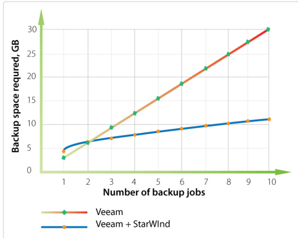
StarWind Global Deduplication Efficiency
